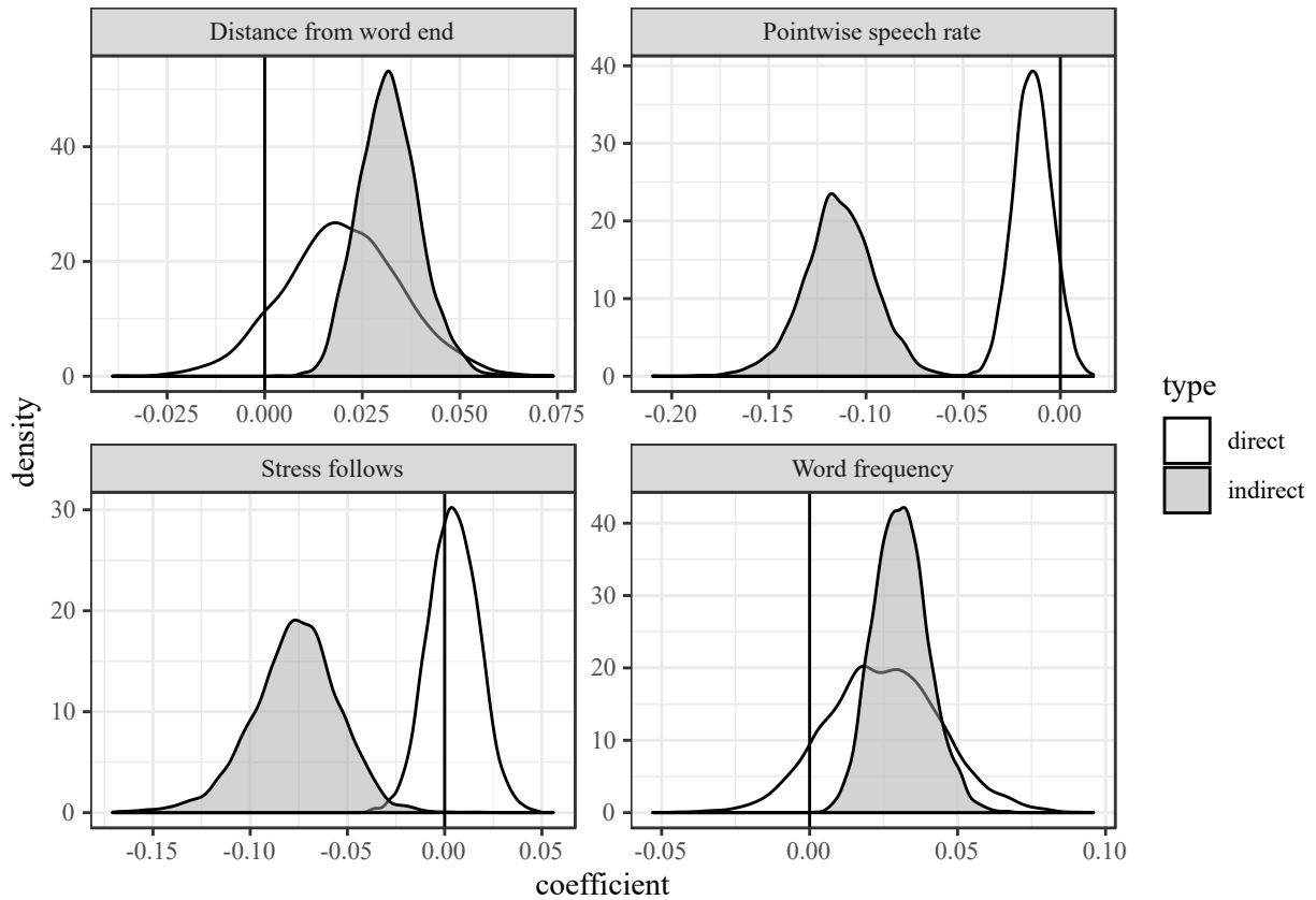
Figure 4: Density plots for the direct and indirect effects of distance from word end, speech rate, whether the following vowel was stressed, and word frequency on relative intensity. Though for all measures the indirect effect is more robust, only speech rate and stress exhibit complete mediation patterns. The indirect path is marked in grey, the direct path is marked in white, and the dark vertical line marks zero (having no effect).
