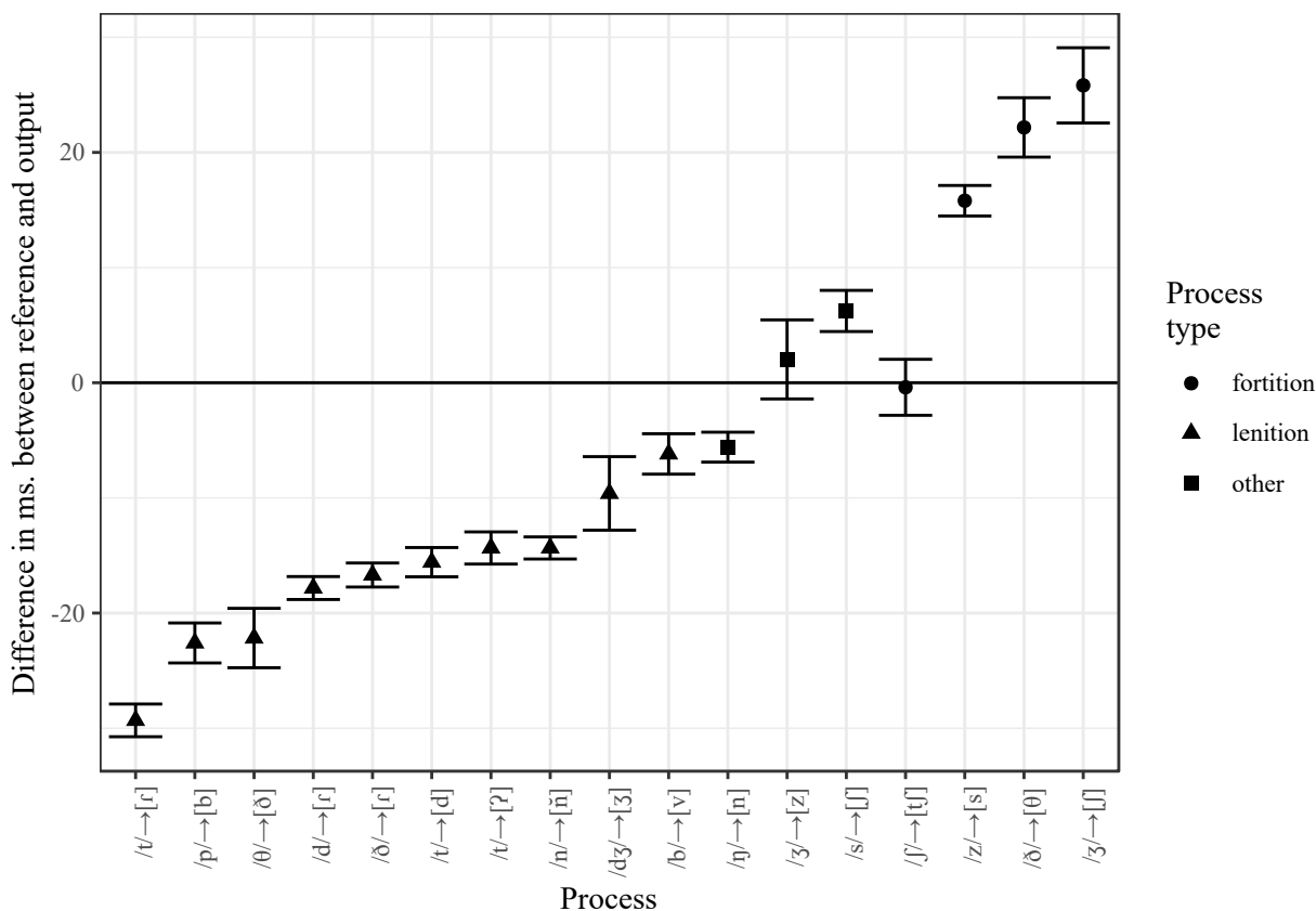
Figure 7: The modeled difference in duration between the surface forms of the two segments involved in a process. The reference segment is treated as a baseline. Negative values indicate that the duration of the output form has shorter duration. Error bars are two standard errors from the mean. Shape indicates the process type (lenition, fortition, or unclassified). The comparison uses the surface method, which ignores the underlying forms of the two segments.
