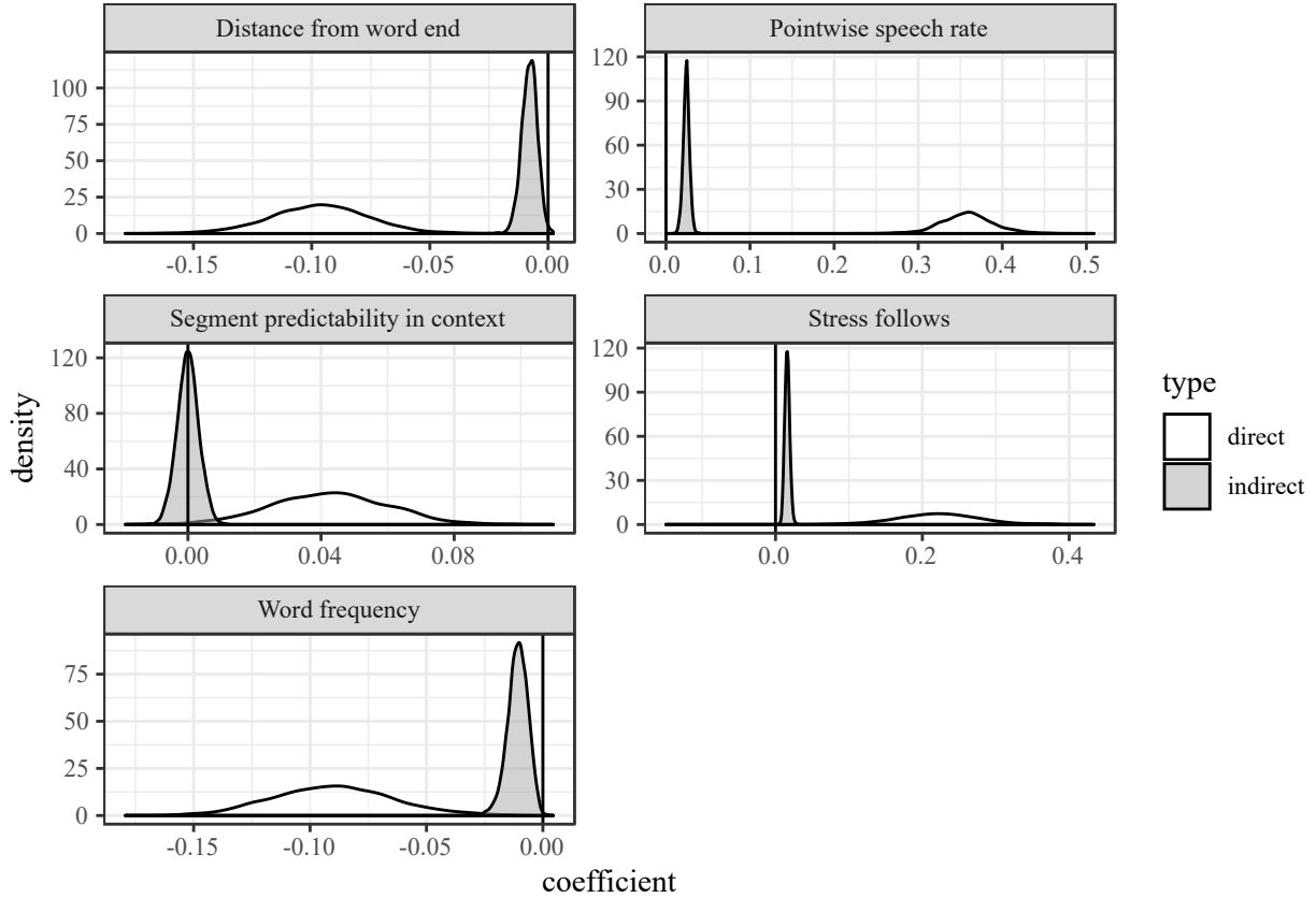
Figure 5: Density plots for the direct and indirect effects of distance from word end, speech rate, whether the following vowel was stressed, and word frequency on relative duration. For all measures the direct effect is more robustly different from zero. The indirect path is marked in grey, the direct path is marked in white, and the dark vertical line marks zero.
