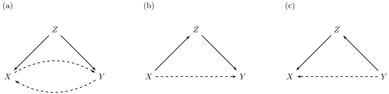
Figure 2: The three possible causal structures for three correlated factors, X , Y , and Z , if X and Y are not correlated when Z is held constant. Dashed lines are causal pathways that are ruled out as impossible by the conditional independence. The figure shows only the direct causation case, but the causal paths are not necessarily direct. In (a) Z causes X and Y , and there is no direct causal link between X and Y . In (b) X causes Z , and Z causes Y , but X does not cause Y except through Z . In (c) Y causes Z , and Z causes X , but Y does not cause X except through Z .
