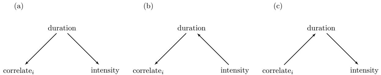
Figure 6: The three possible causal structures given the results of Study 1, for each of the correlates. “Correlate i ” stands for any of the correlates of lenition, “duration” stands for changes in duration, and “intensity” stands for changes in intensity. In each alternative, the lines represent (jointly) a possible causal relationship. In (a), changes in duration cause the correlate and changes in intensity. In (b), changes in intensity cause changes in duration, and changes in duration cause changes in the correlate. In (c), the correlate causes changes in duration, and changes in duration cause changes in intensity. For different correlates correlate k and correlate j , (a) and (c) are compatible, as the causal direction between duration and intensity does not change. However, (a) and (c) are not compatible with (b) because the causal direction between direction and intensity is reversed.
